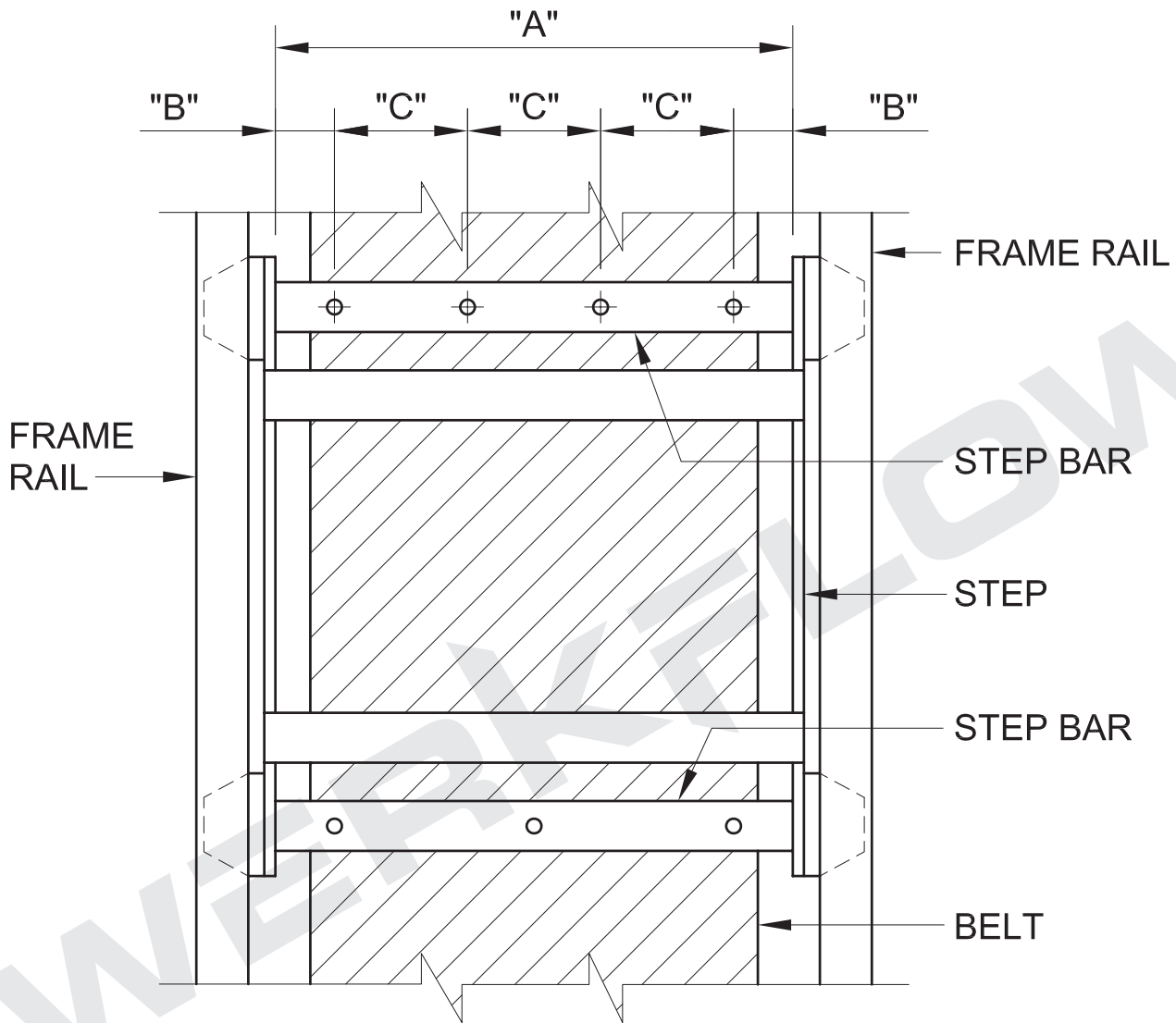
FACING BELT - VIEW
